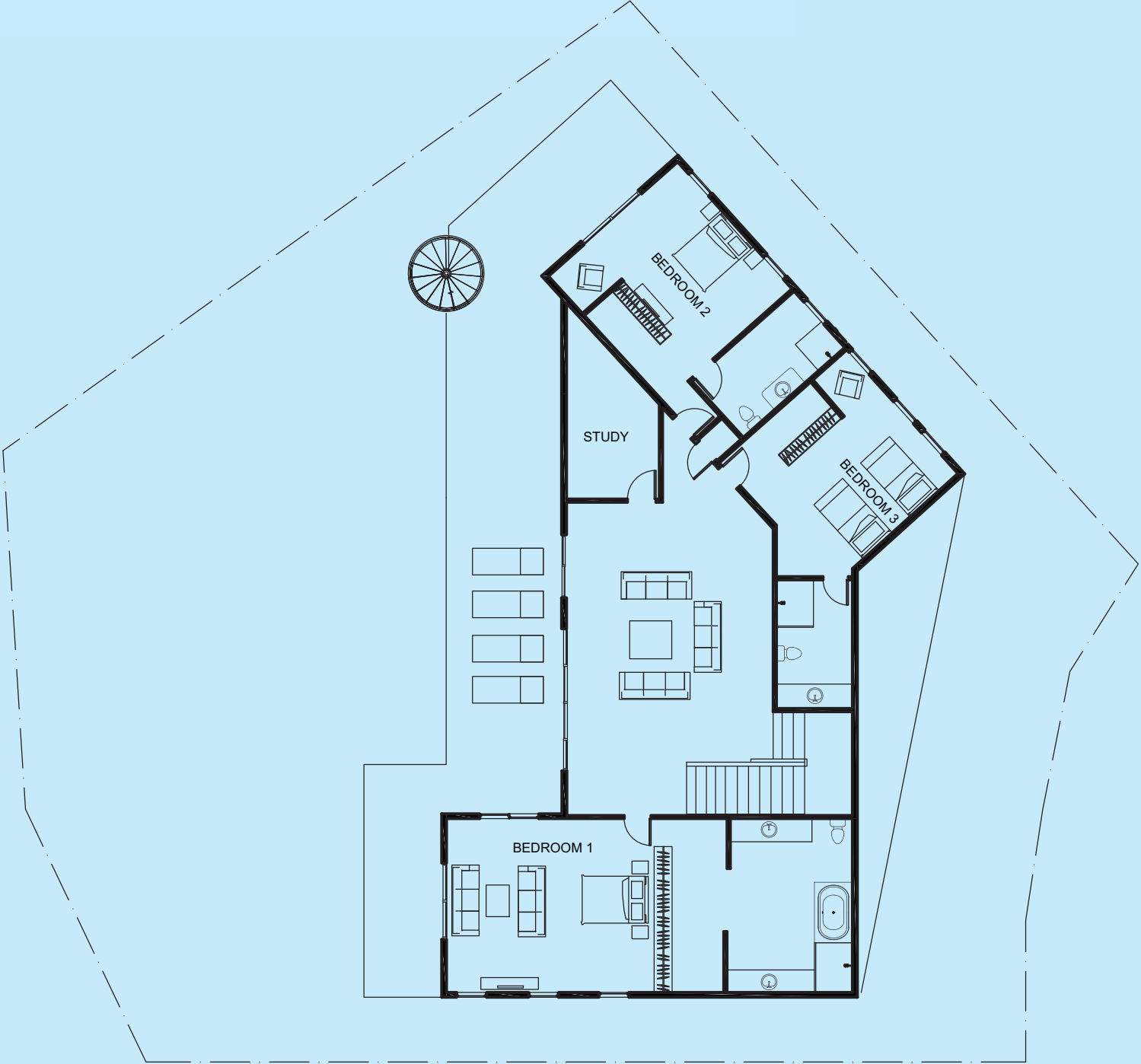
DIAMOND UPPER LEVEL FLOOR PLAN
